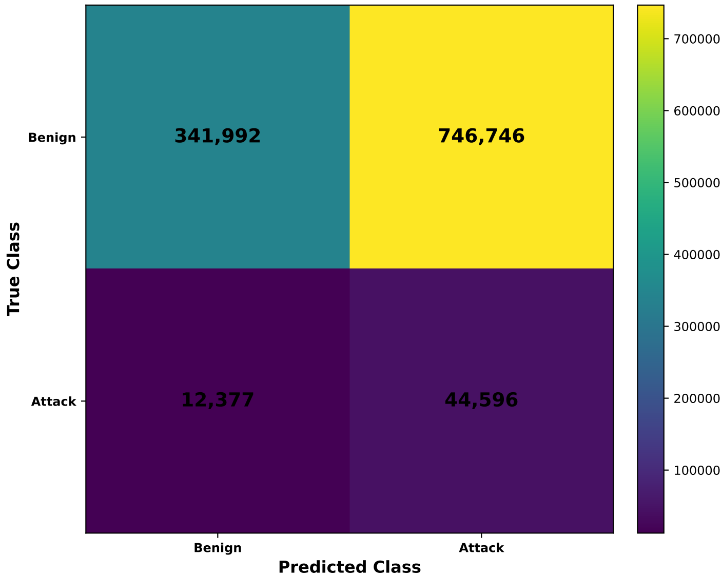
XGBoost Compact Binary Validation Confusion Matrix
