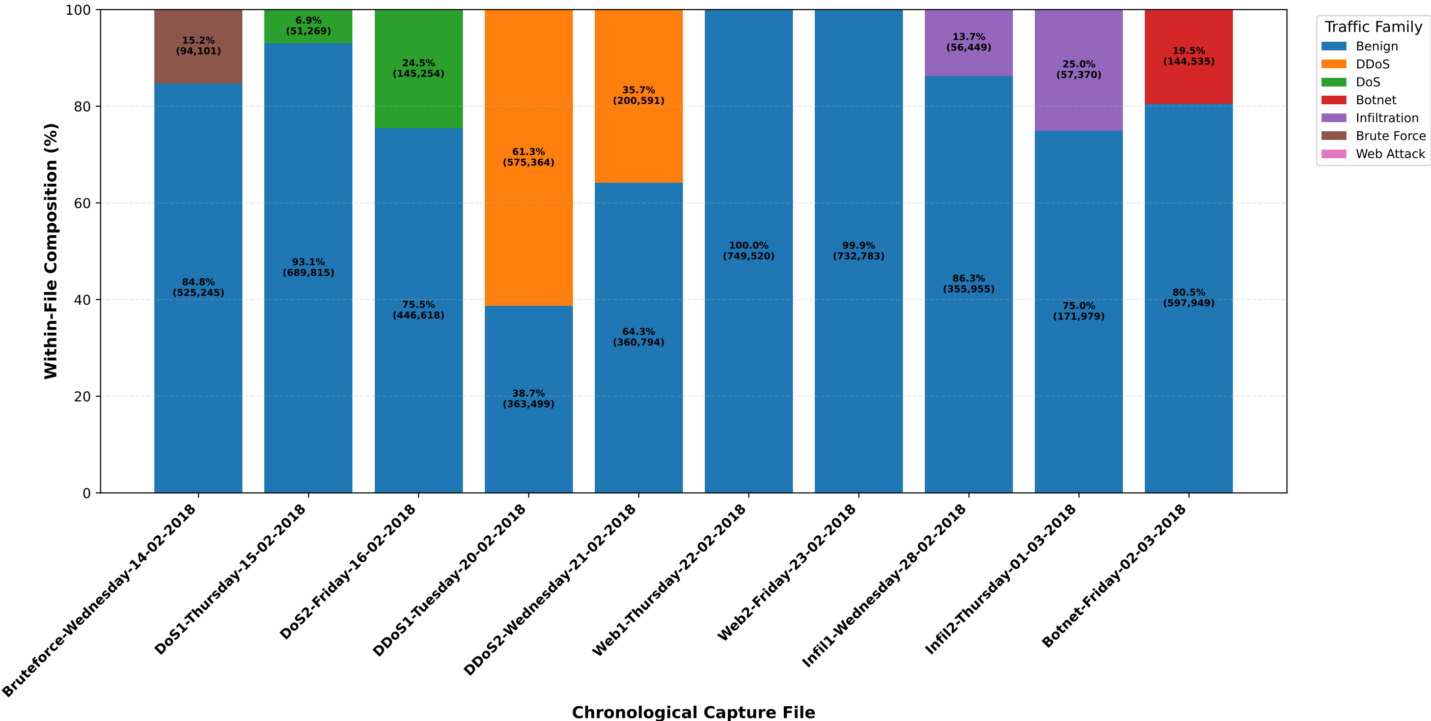
Chronological Traffic-Family Composition After Deduplication
