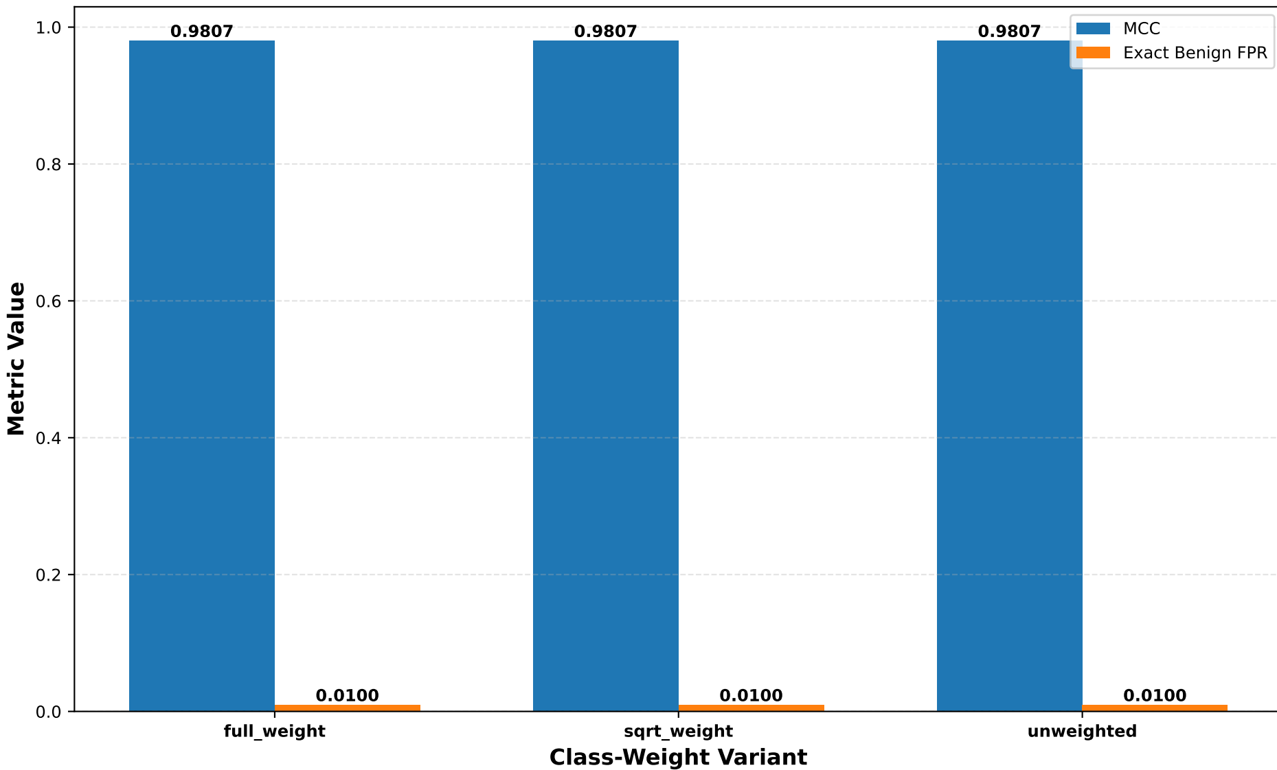
CatBoost GPU Class-Weight Ablation at FPR \leq 1%
