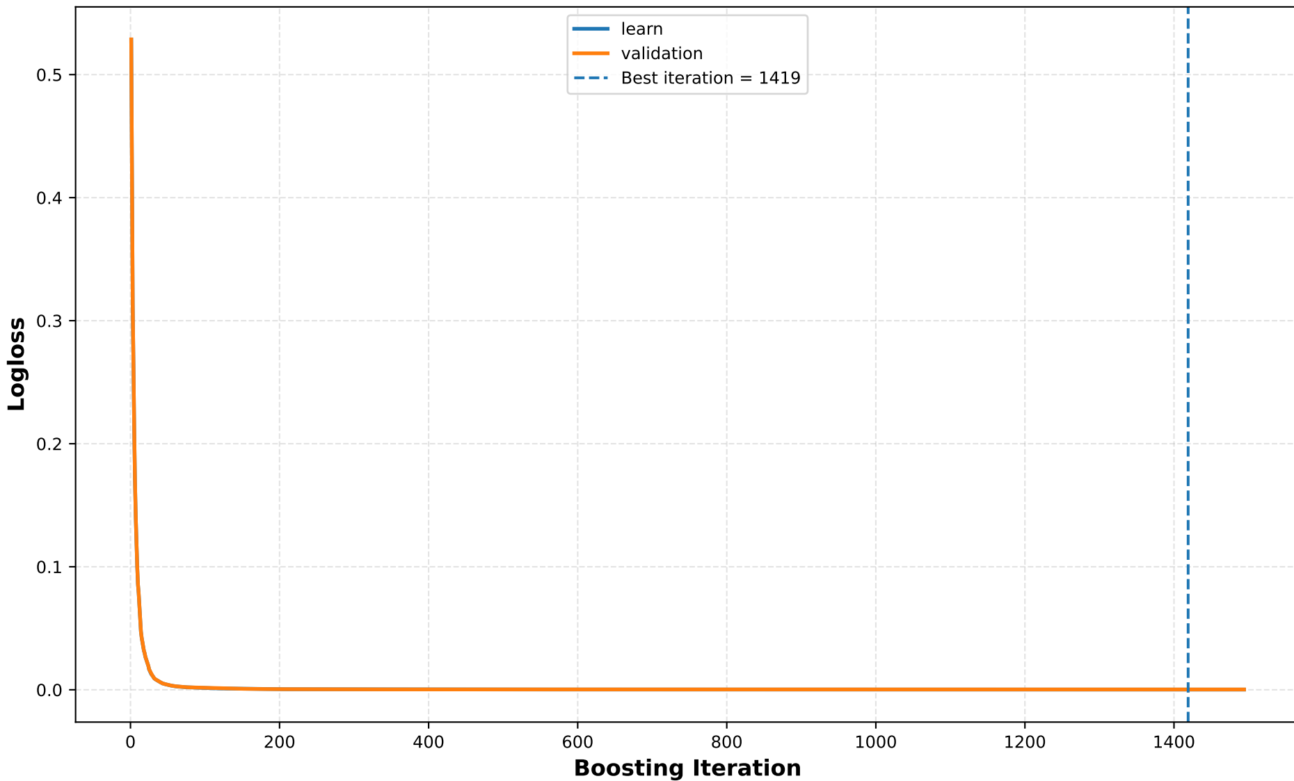
Selected CatBoost Training and Holdout Log-Loss
