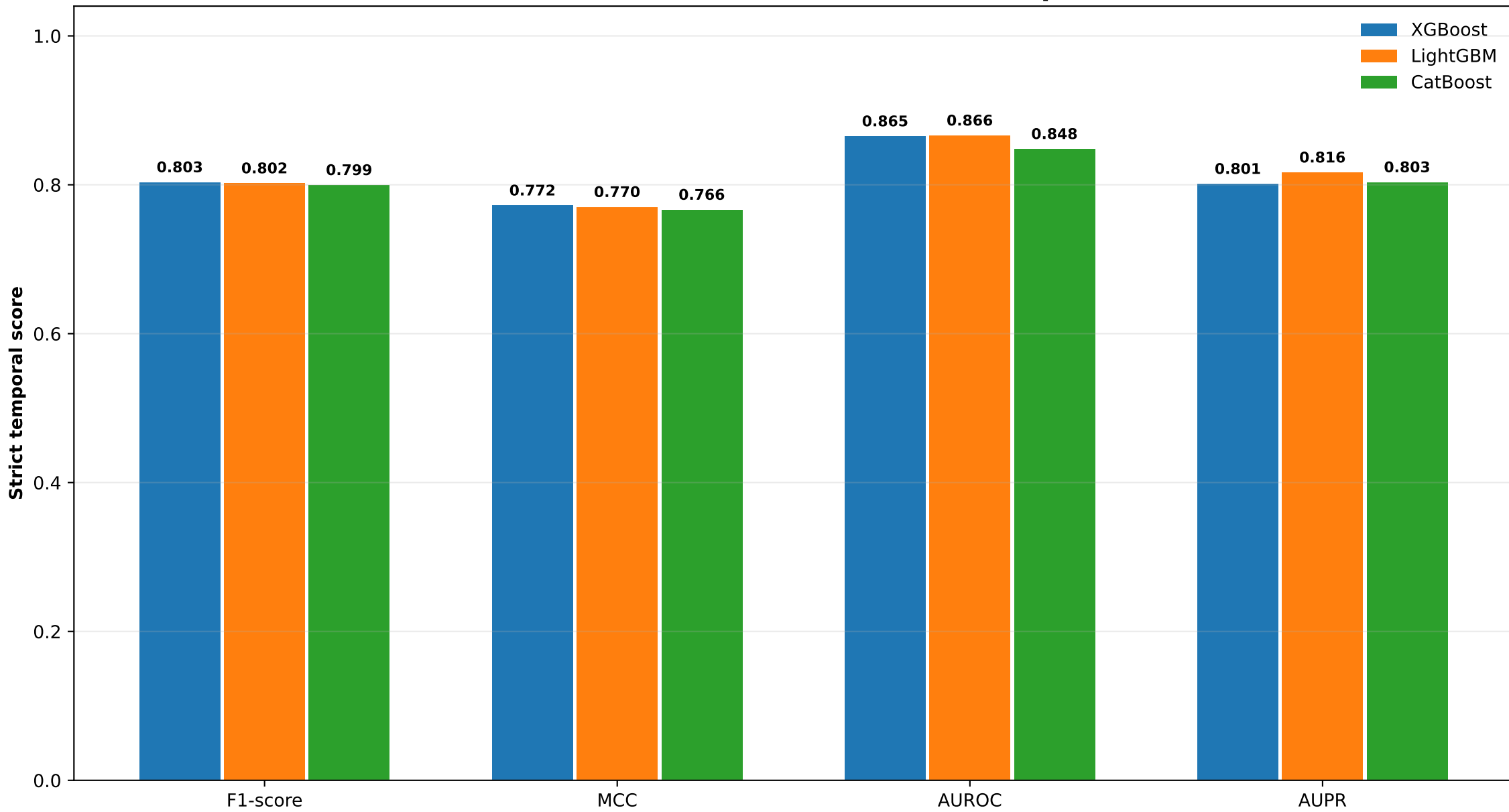
Tree-Based Intrusion Detection: Strict Temporal Test
