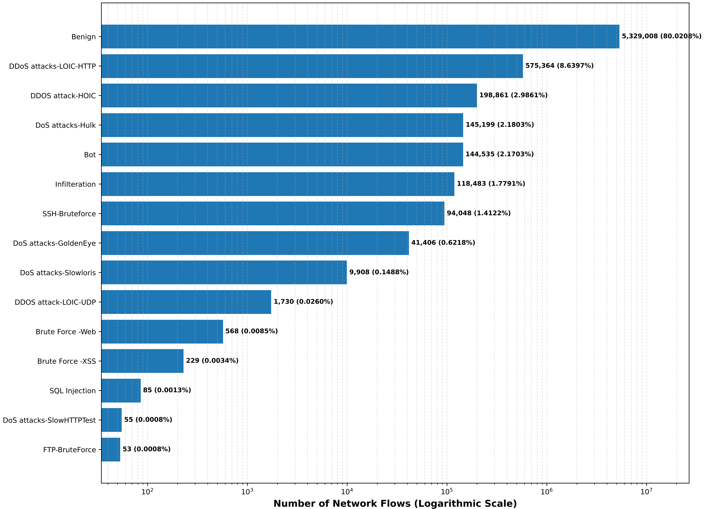
Global Class Distribution of CSE-CIC-IDS2018
