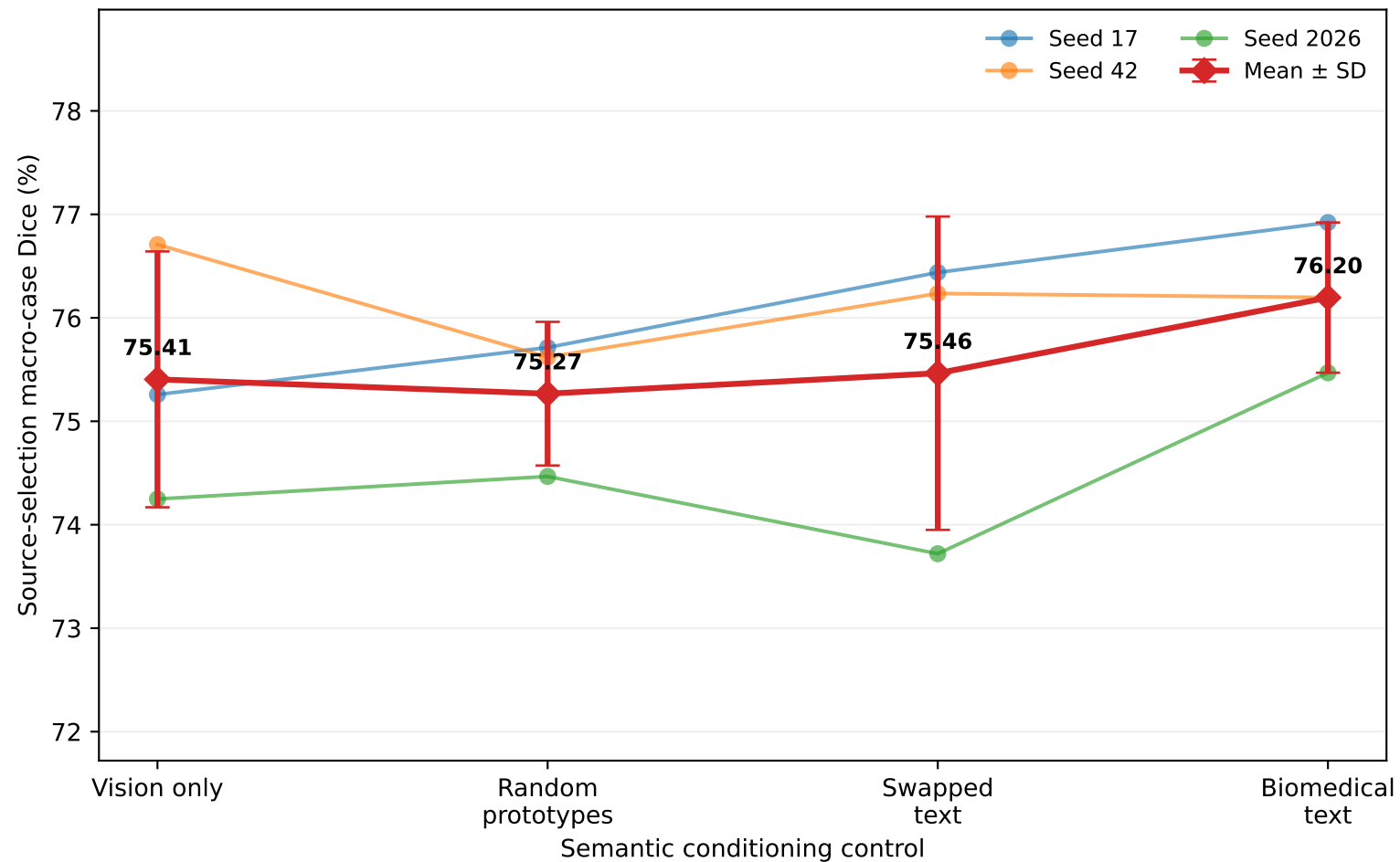
Semantic Ablation: Biomedical Text vs Matched Controls
