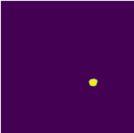
Probability
