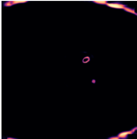
Uncertainty
