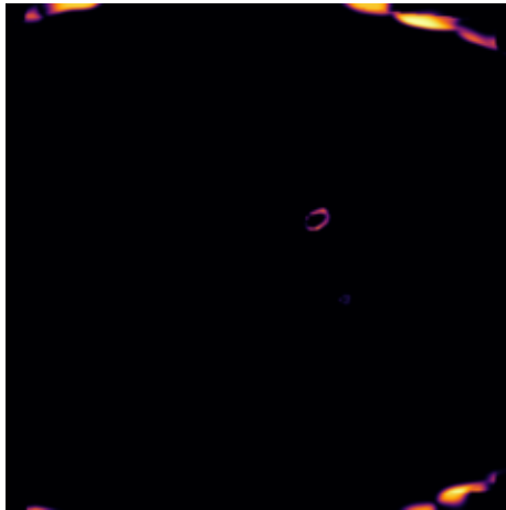
View variance
