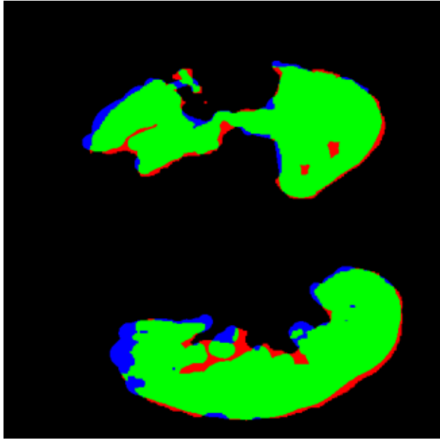
Agreement Error
