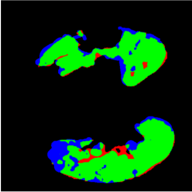
Supervised Error
