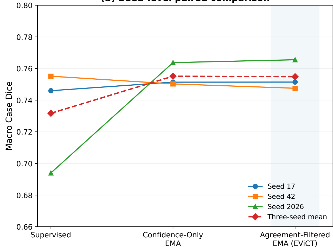
(b) Seed-level paired comparison
