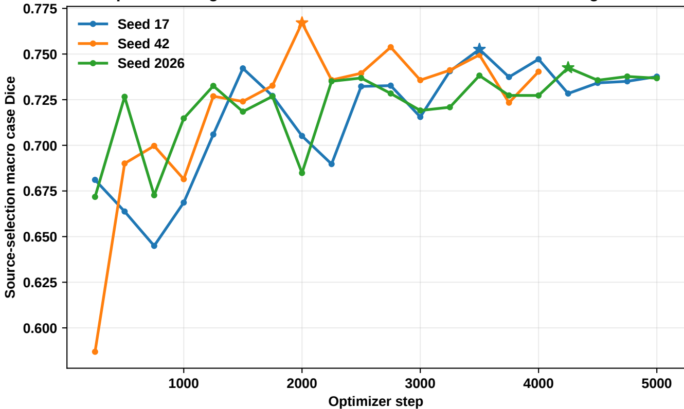
Supervised SegFormer-B1: three-seed source-selection learning curves
