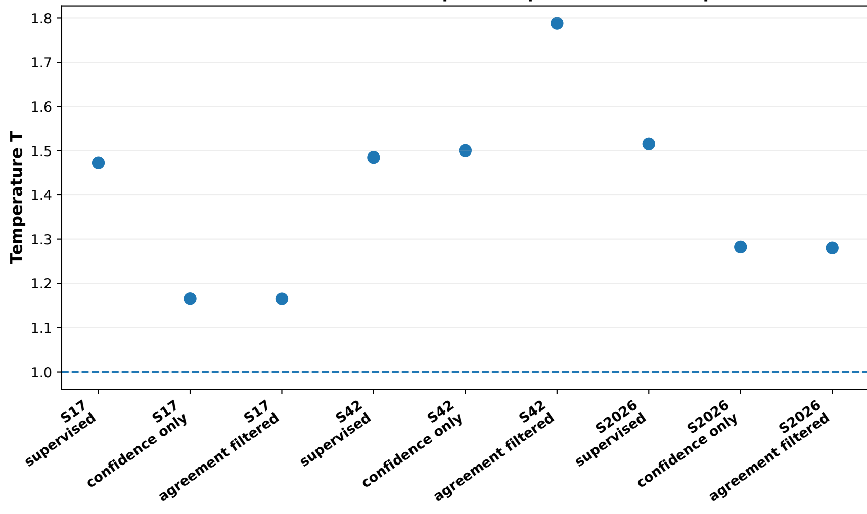
Final Source-Calibration Temperature per Selected Checkpoint
