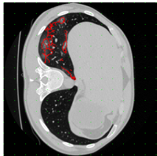
Sparse Scribble
