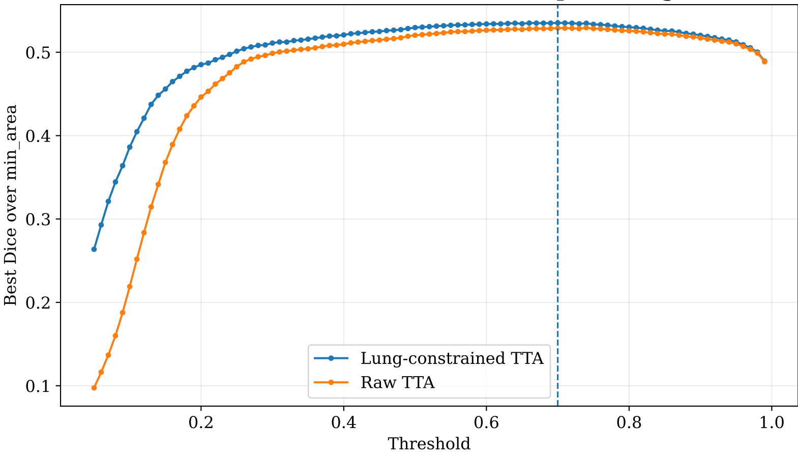
MosMed Fine-tuned Teacher: TTA + Post-processing Search
