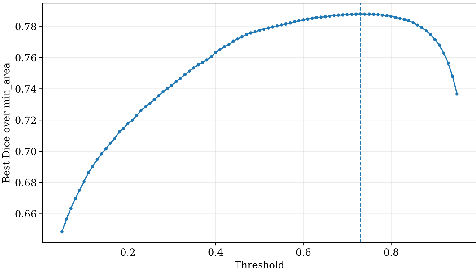
COVID Lesion CASR-Net Teacher-Initialized Validation Search
