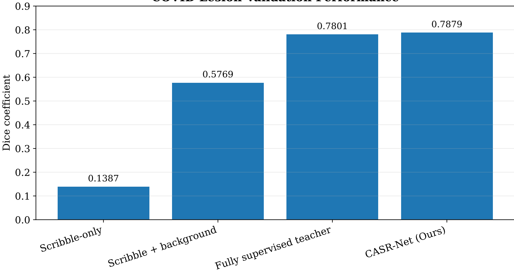
COVID Lesion Validation Performance
