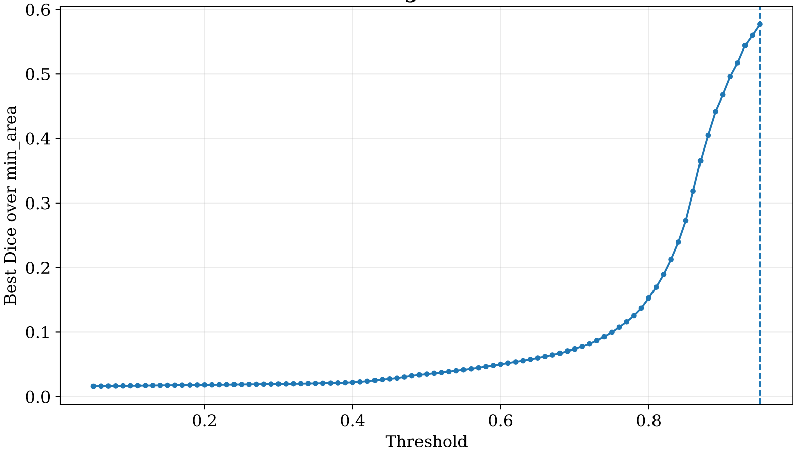
COVID Lesion Scribble + Background Baseline Validation Search
