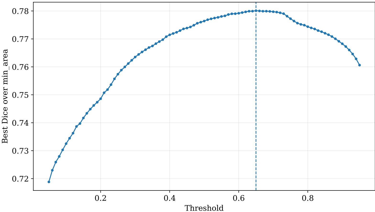
COVID Lesion Teacher Validation Search
