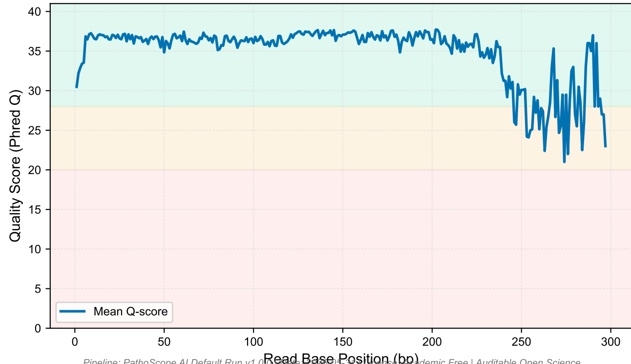
Per-Base Sequence Quality Distribution (Line shows mean Phred Q scores across query reads)
