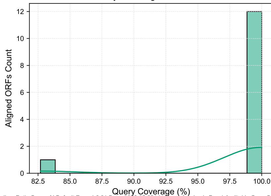
Query Coverage Distribution
