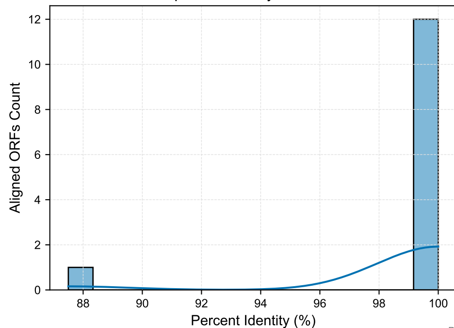
Sequence Identity Distribution
