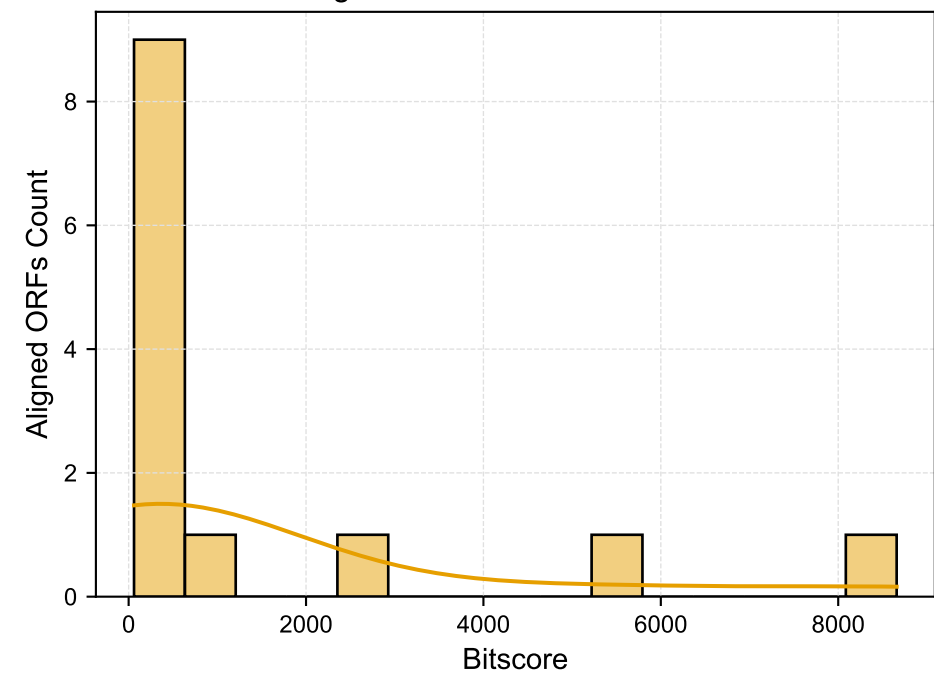
Alignment Bitscore Distribution
