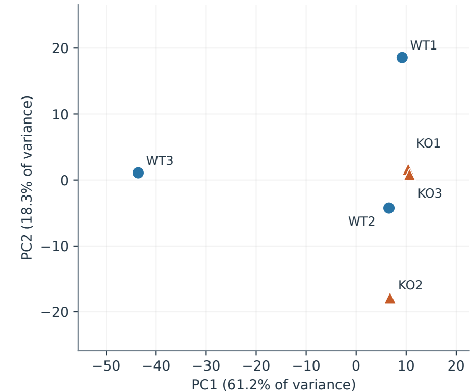
A PCA: 500 most variable genes
