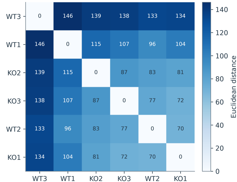
B Sample distances: all retained genes
