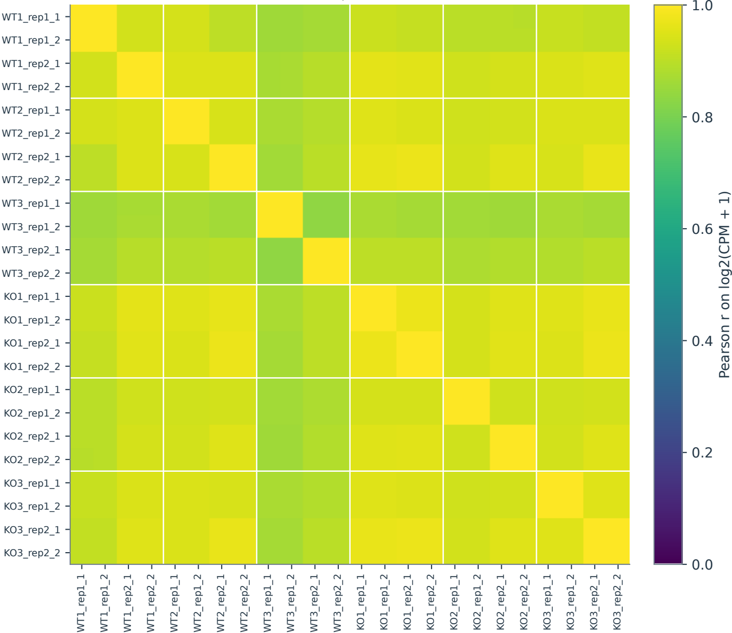
B Technical-file expression correlations
