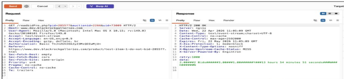
Fig: Shows server send current bid value even without any session cookie
