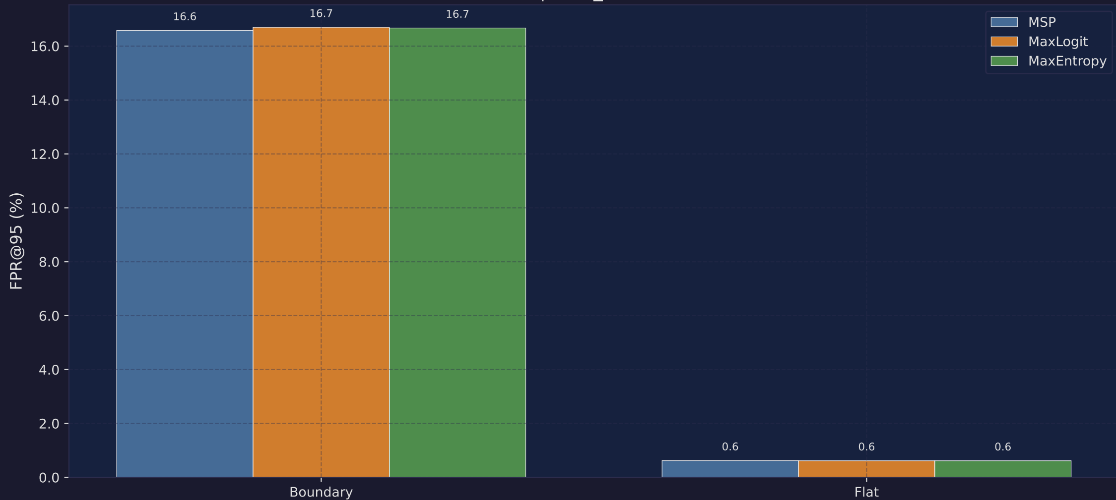
FPR@95 — Boundary vs Flat Region EoMT | road_obstacle21
