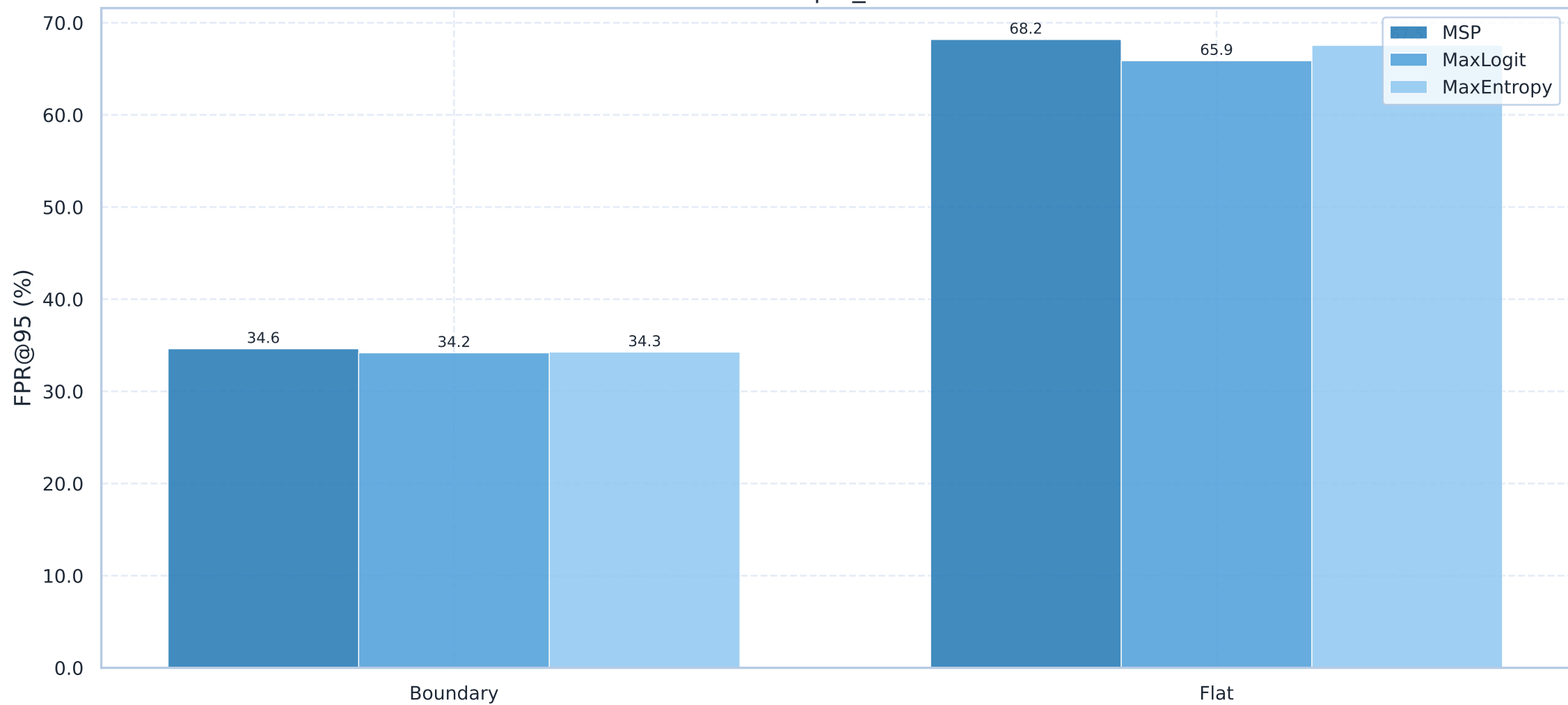
FPR@95 - Boundary vs Flat Region EoMT | fs_static
