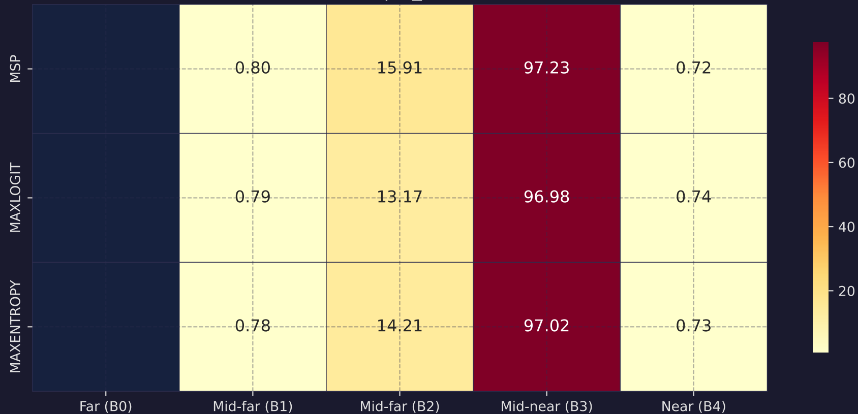
FPR@95 (%) by Depth Band EoMT | fs_static
