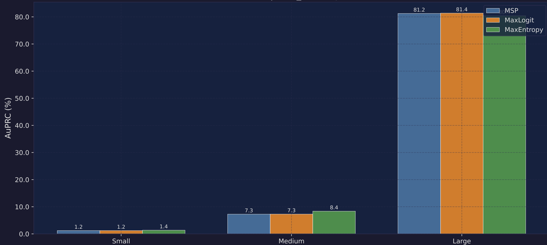
AuPRC by Anomaly Size Bucket EoMT | road_anomaly
