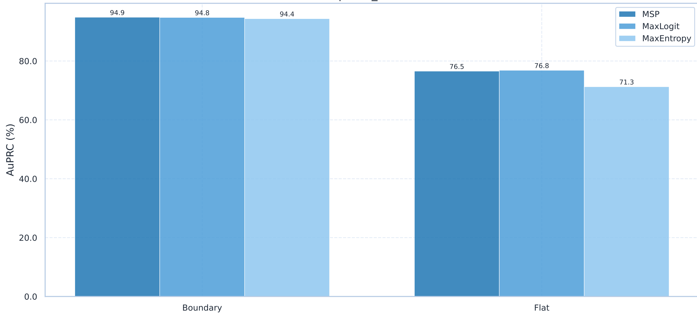
AuPRC - Boundary vs Flat Region EoMT | road_obstacle21
