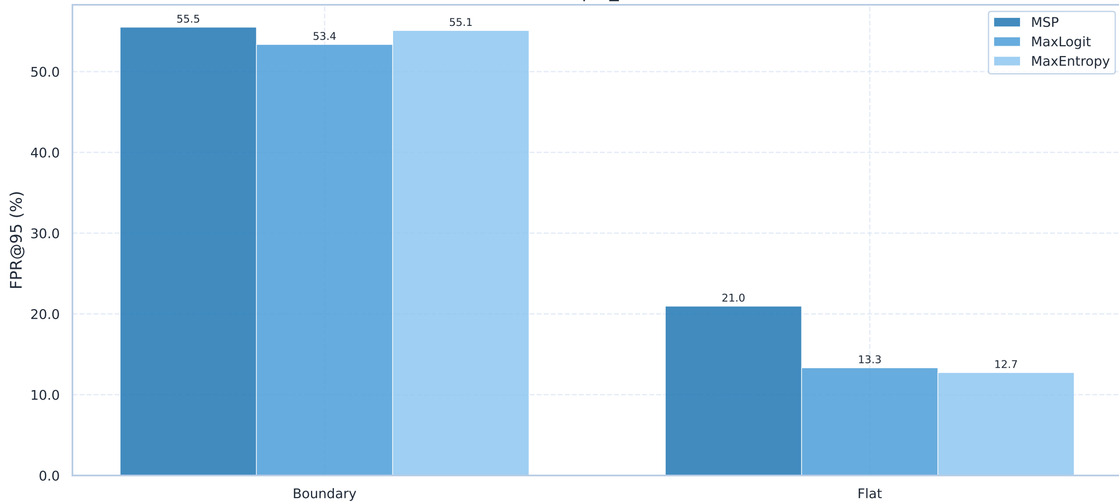
FPR@95 - Boundary vs Flat Region EoMT | fs_static
