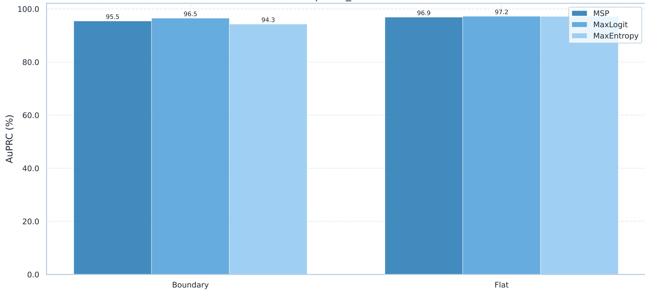
AuPRC - Boundary vs Flat Region EoMT | road_obstacle21
