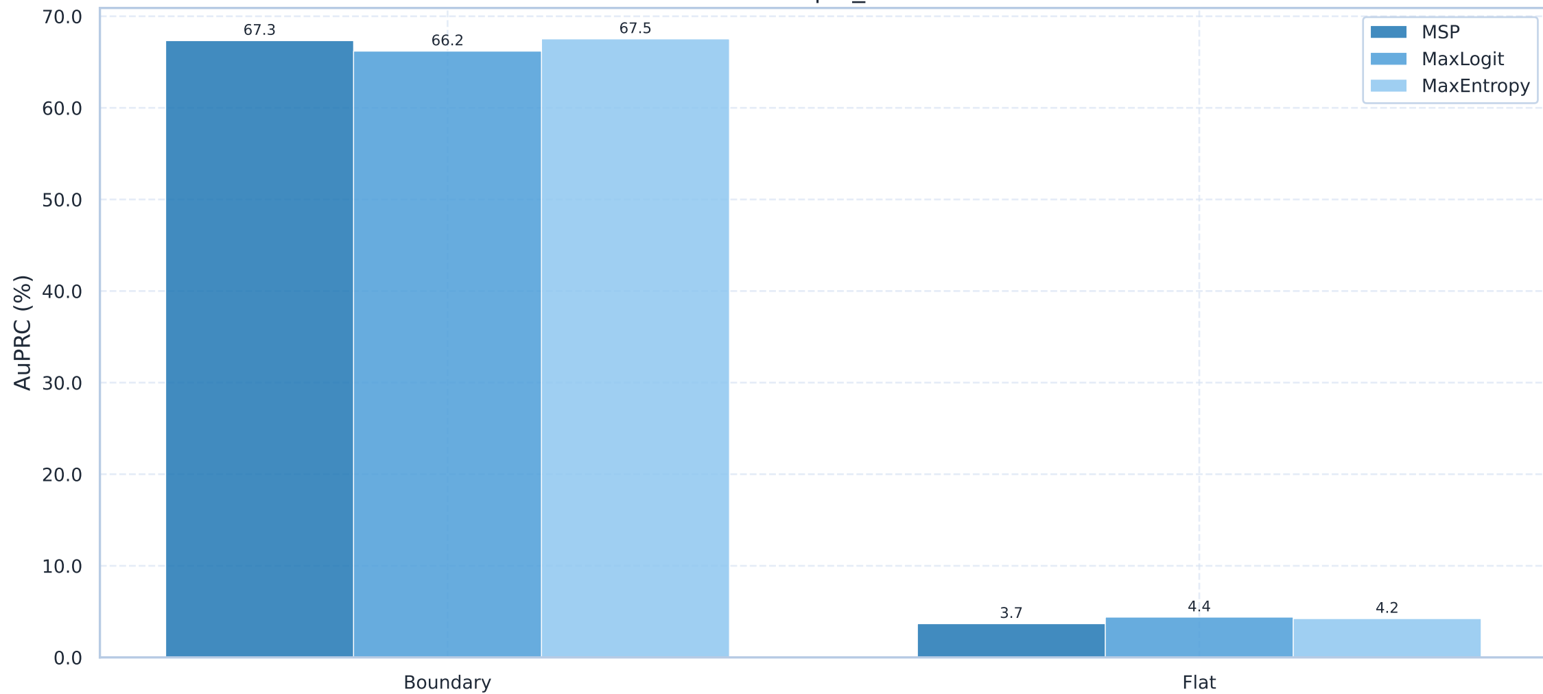
AuPRC - Boundary vs Flat Region ERFNet | fs_static
