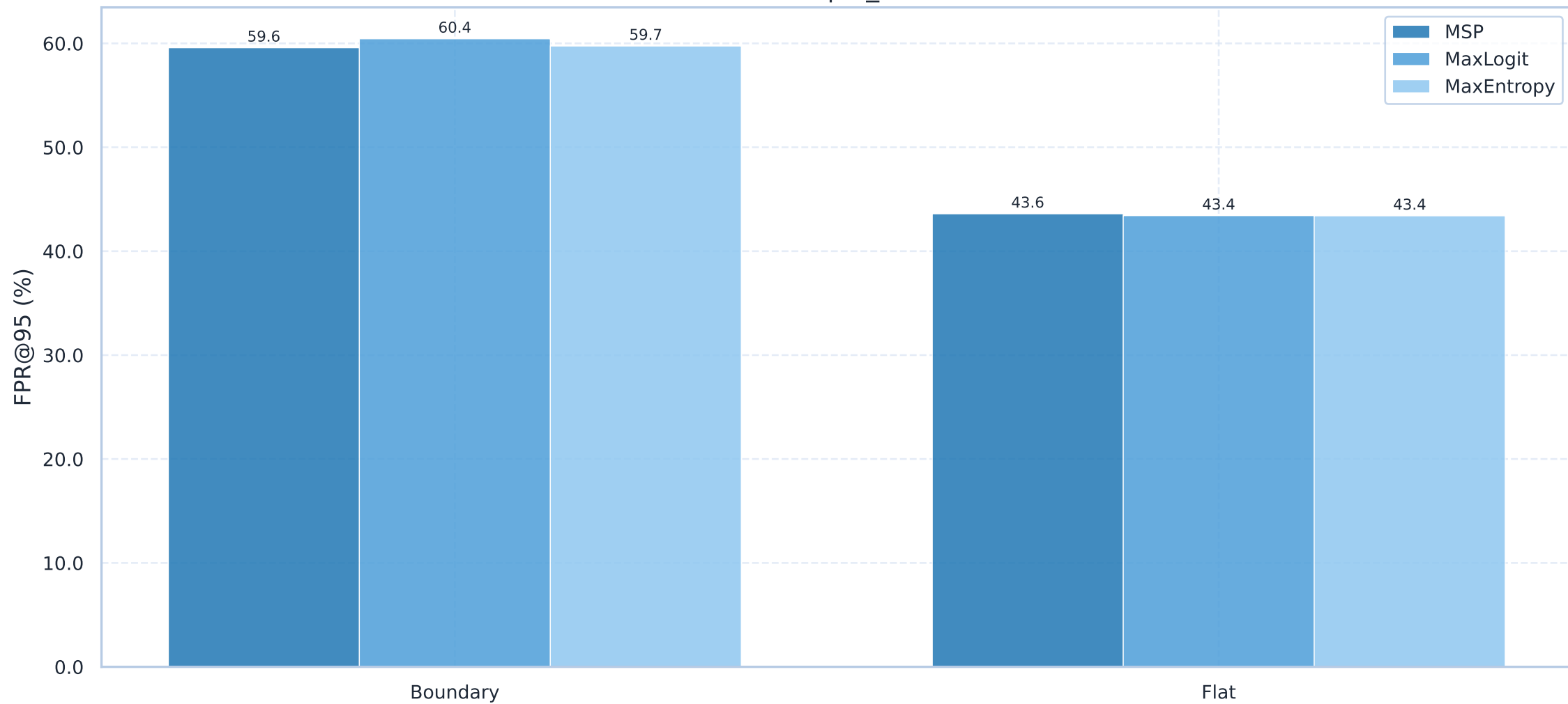
FPR@95 - Boundary vs Flat Region ERFNet | fs_static
