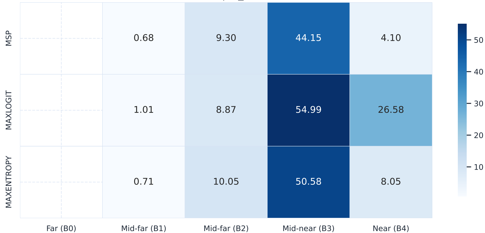
AuPRC (%) by Depth Band ERFNet | fs_static
