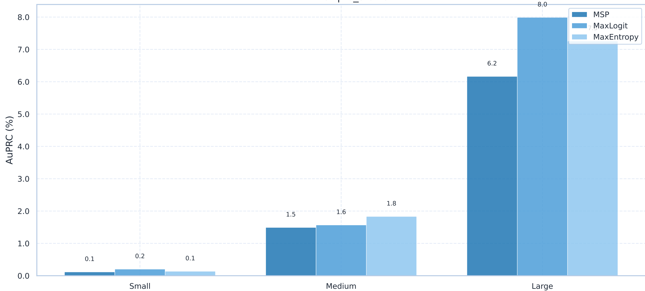
AuPRC by Anomaly Size Bucket ERFNet | fs_static
