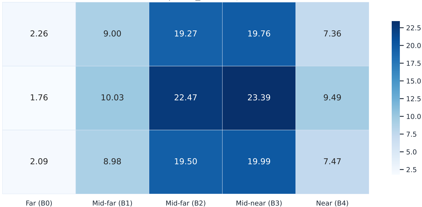
AuPRC (%) by Depth Band ERFNet | road_anomaly
