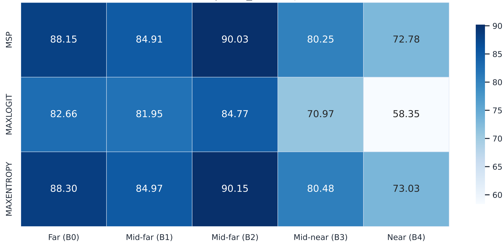
FPR@95 (%) by Depth Band ERFNet | road_anomaly
