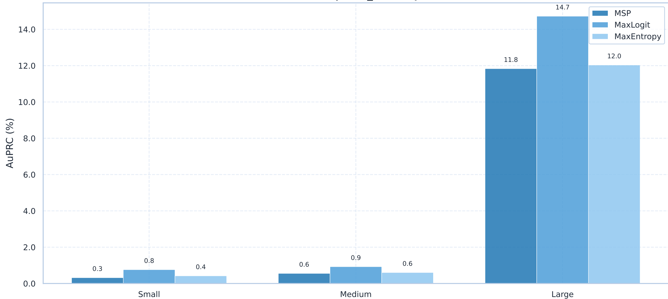
AuPRC by Anomaly Size Bucket ERFNet | road_anomaly
