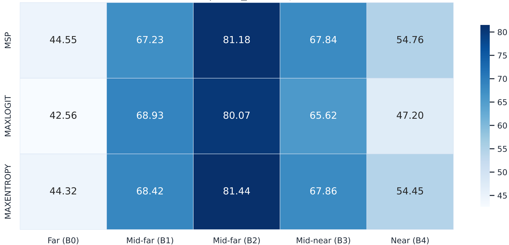
FPR@95 (%) by Depth Band ERFNet | road_anomaly21
