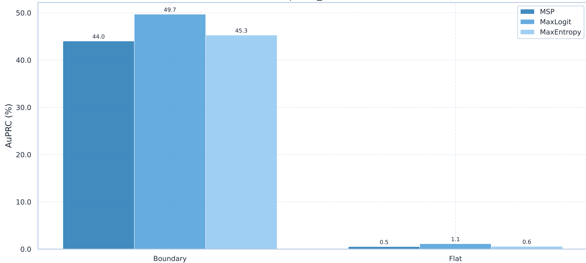
AuPRC - Boundary vs Flat Region ERFNet | road_obstacle21
