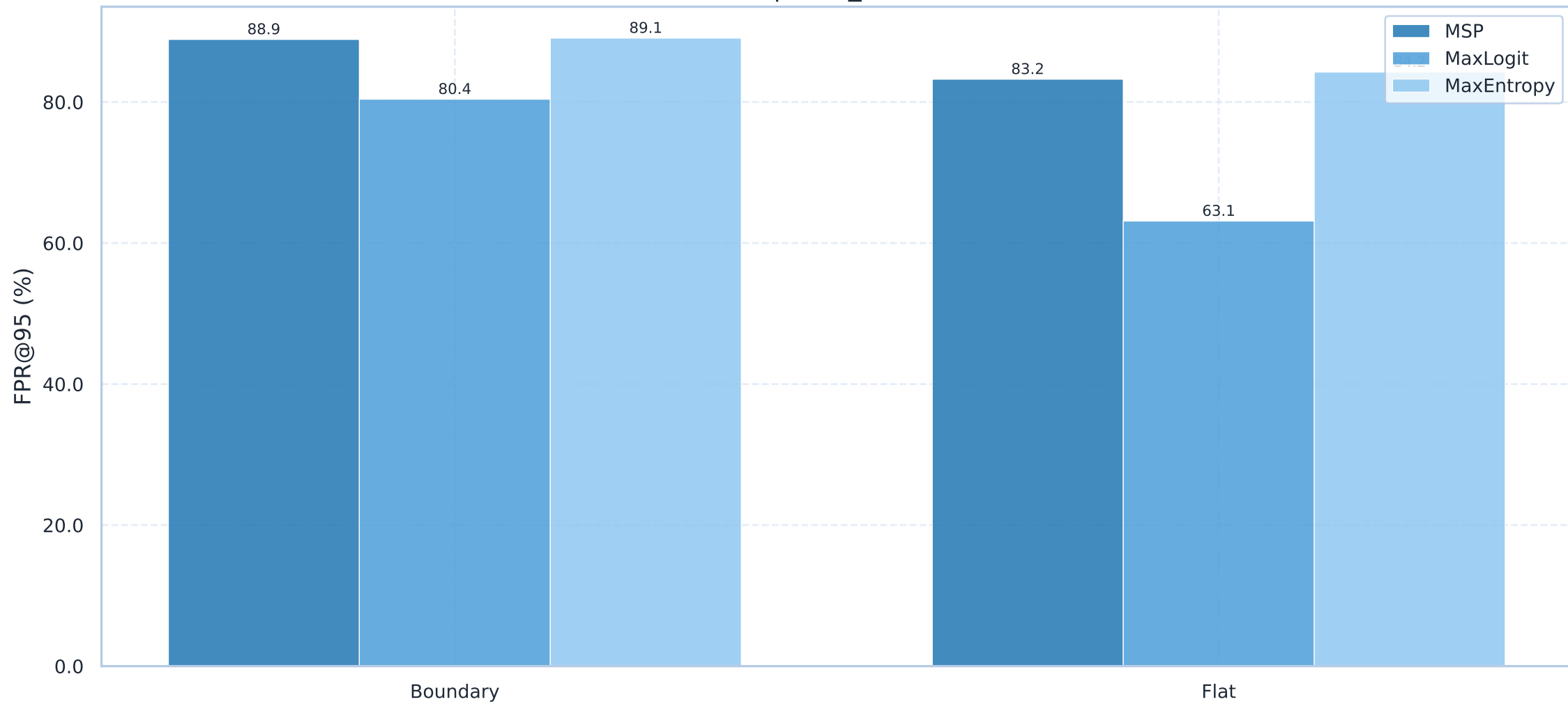
FPR@95 - Boundary vs Flat Region ERFNet | road_obstacle21
