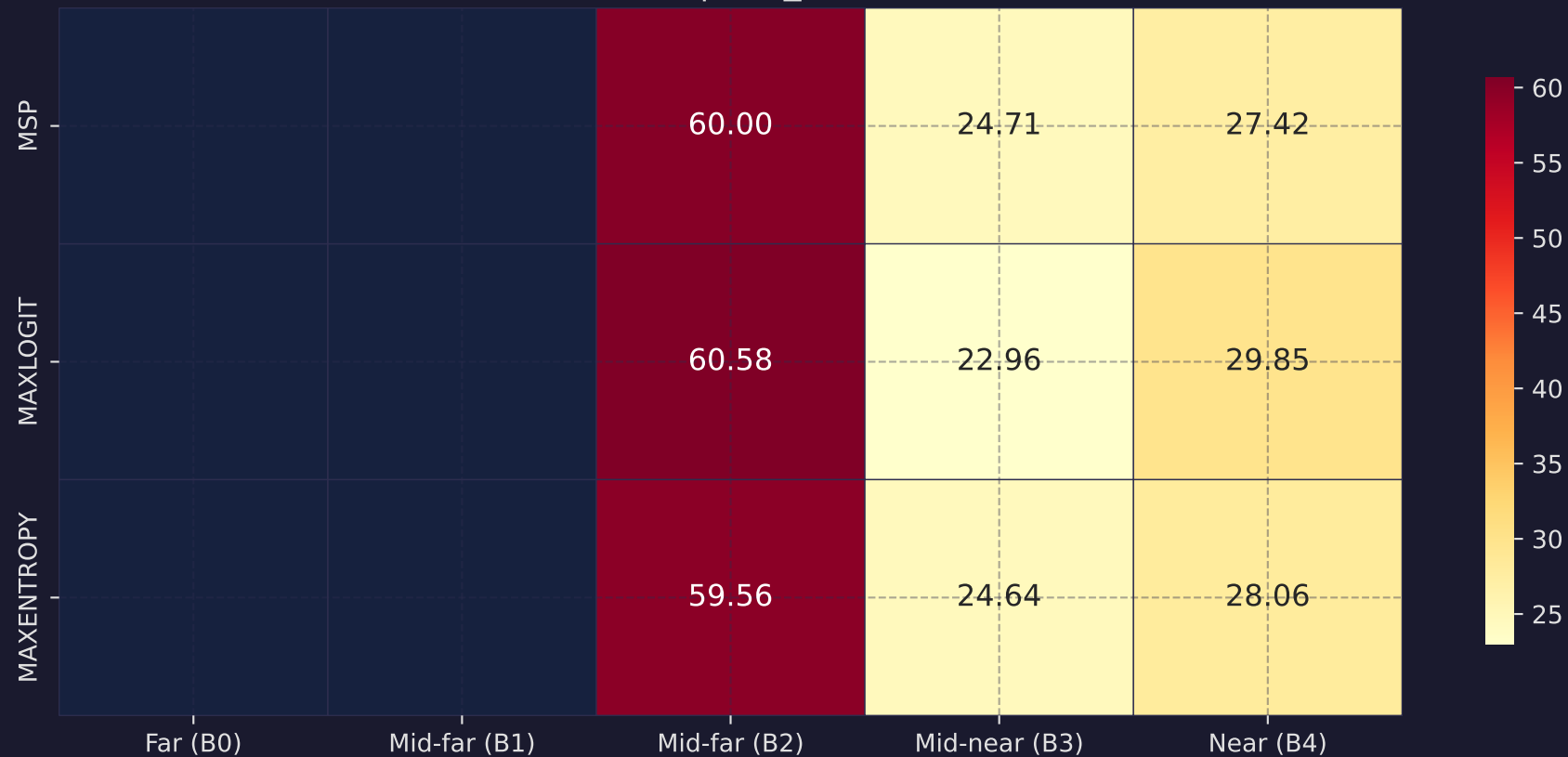
FPR@95 (%) by Depth Band ERFNet | lost_found
