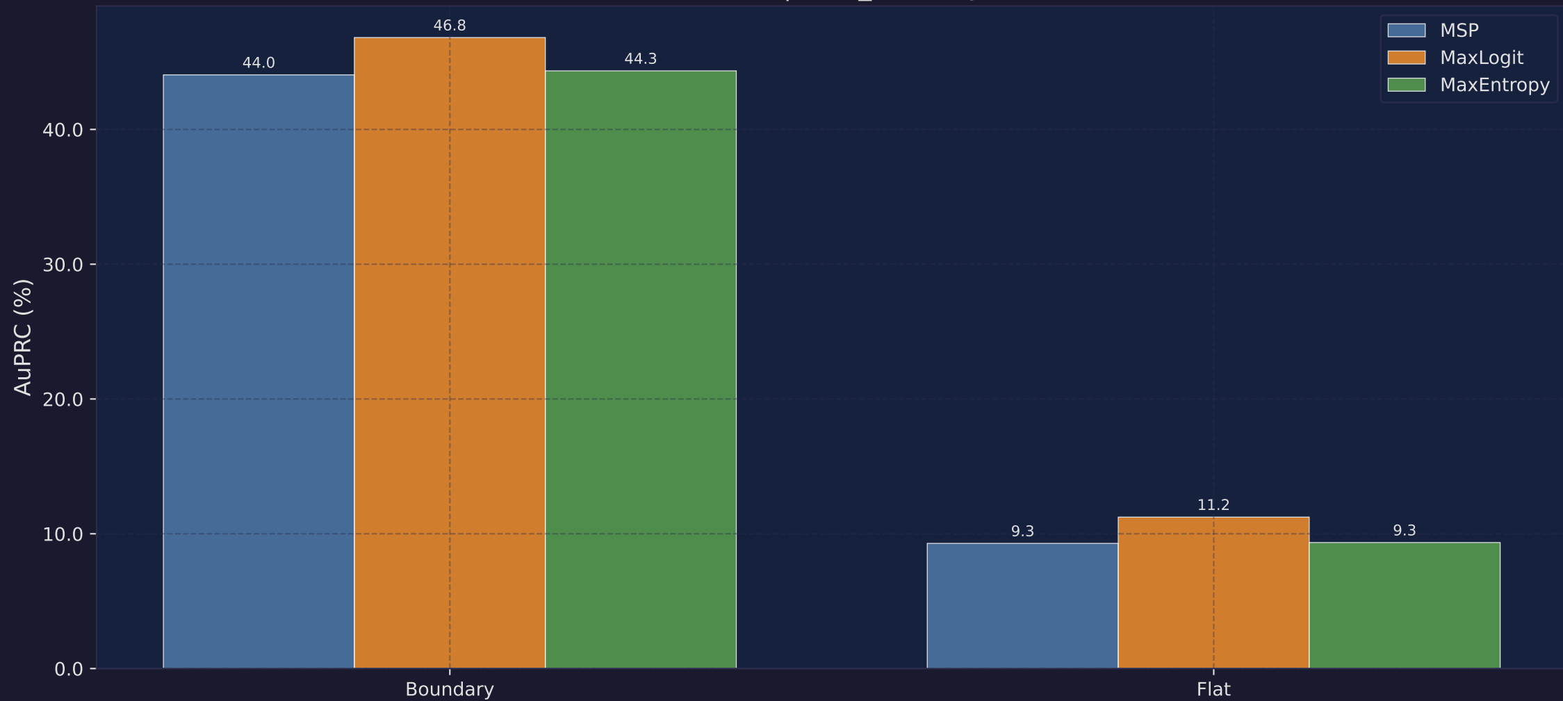
AuPRC — Boundary vs Flat Region ERFNet | road_anomaly
