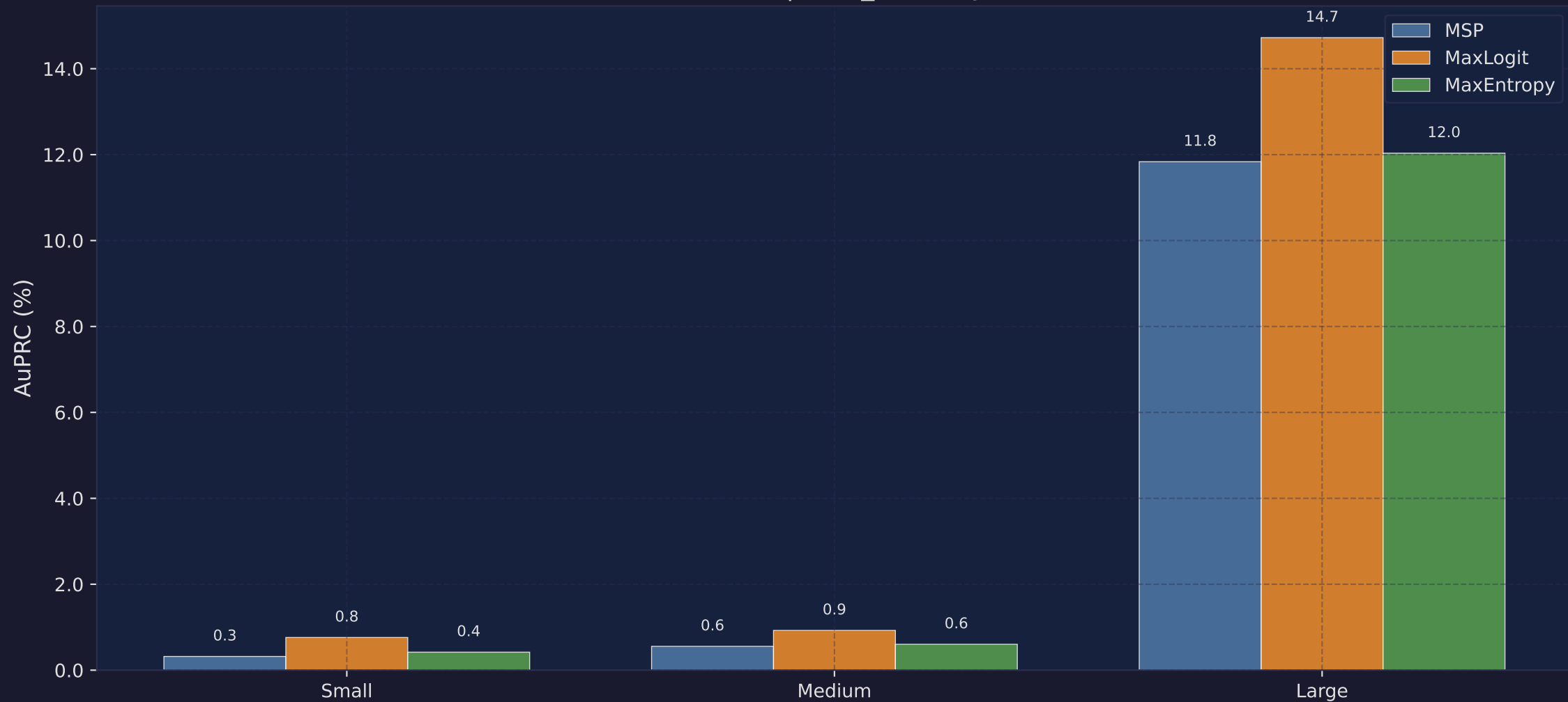
AuPRC by Anomaly Size Bucket ERFNet | road_anomaly
