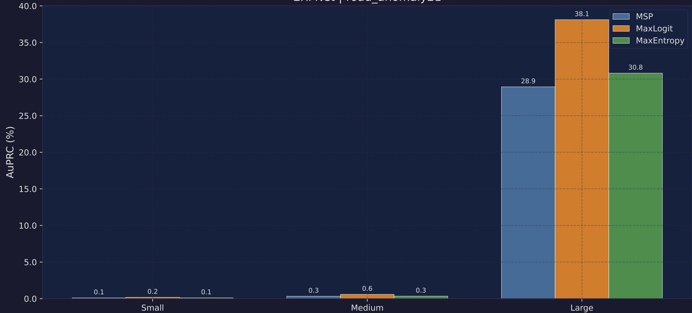
AuPRC by Anomaly Size Bucket ERFNet | road_anomaly21
