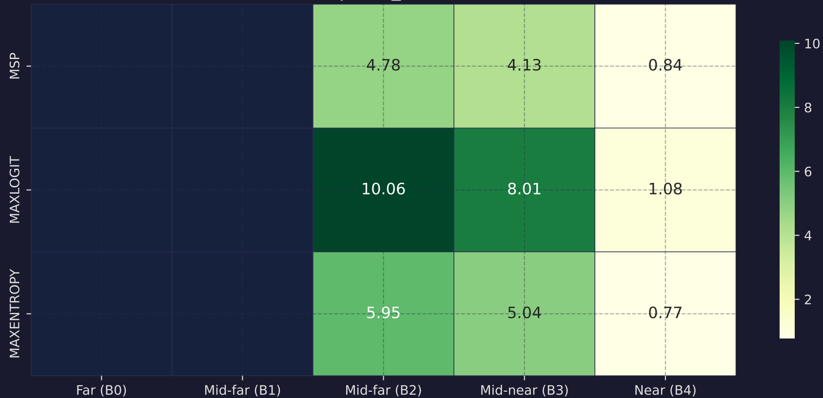
AuPRC (%) by Depth Band ERFNet | road_obstacle21
