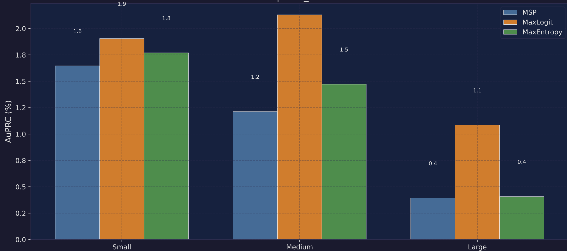
AuPRC by Anomaly Size Bucket ERFNet | road_obstacle21
