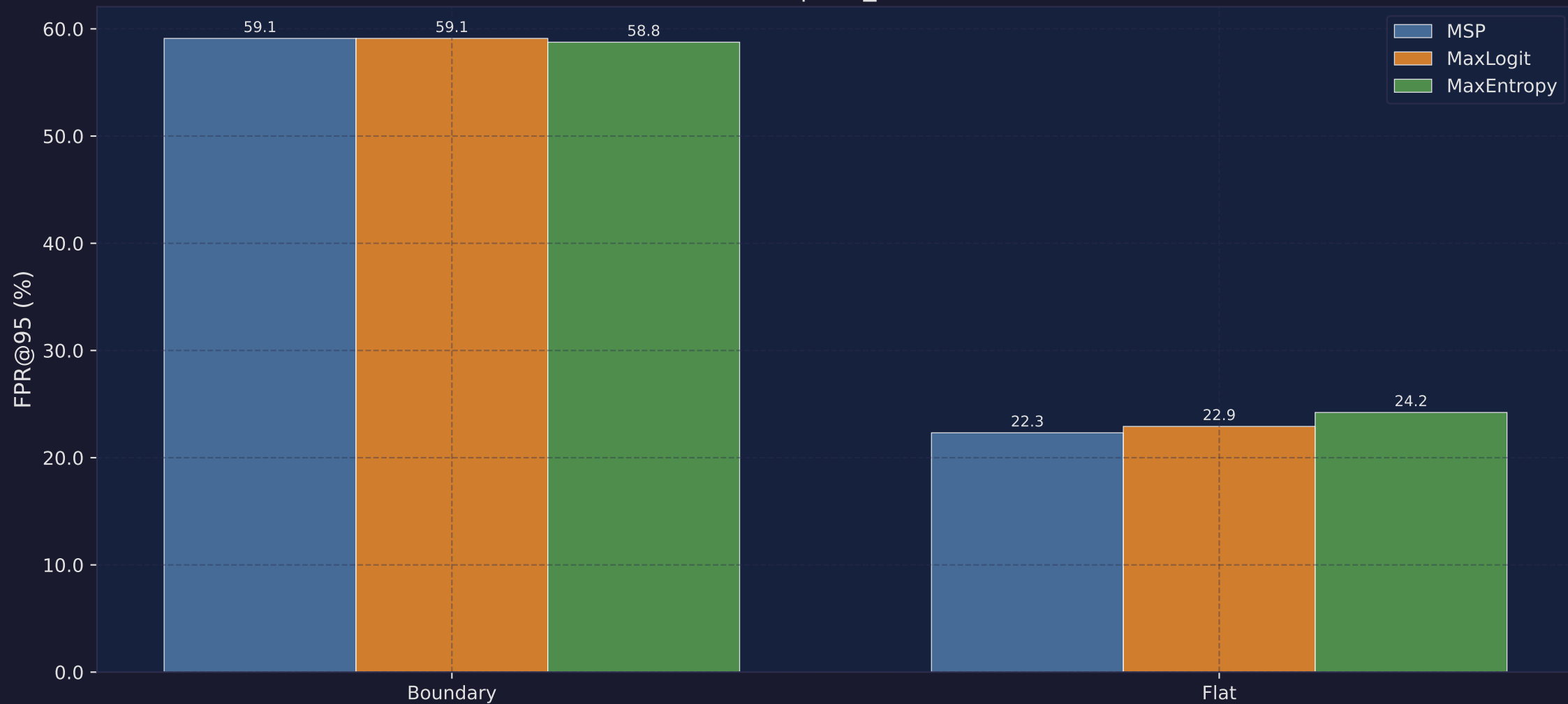
FPR@95 — Boundary vs Flat Region EoMT | lost_found
