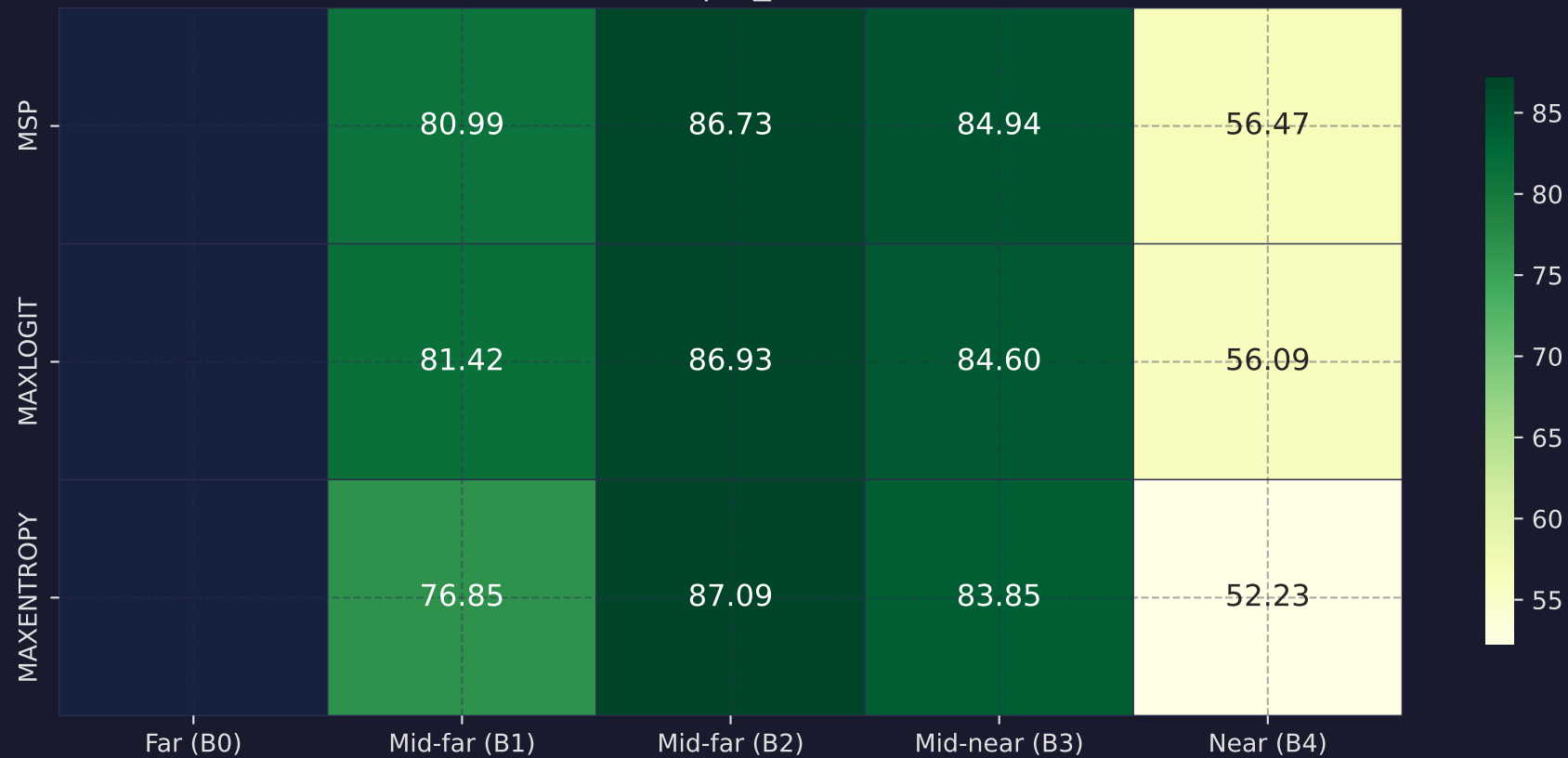
AuPRC (%) by Depth Band EoMT | fs_static
