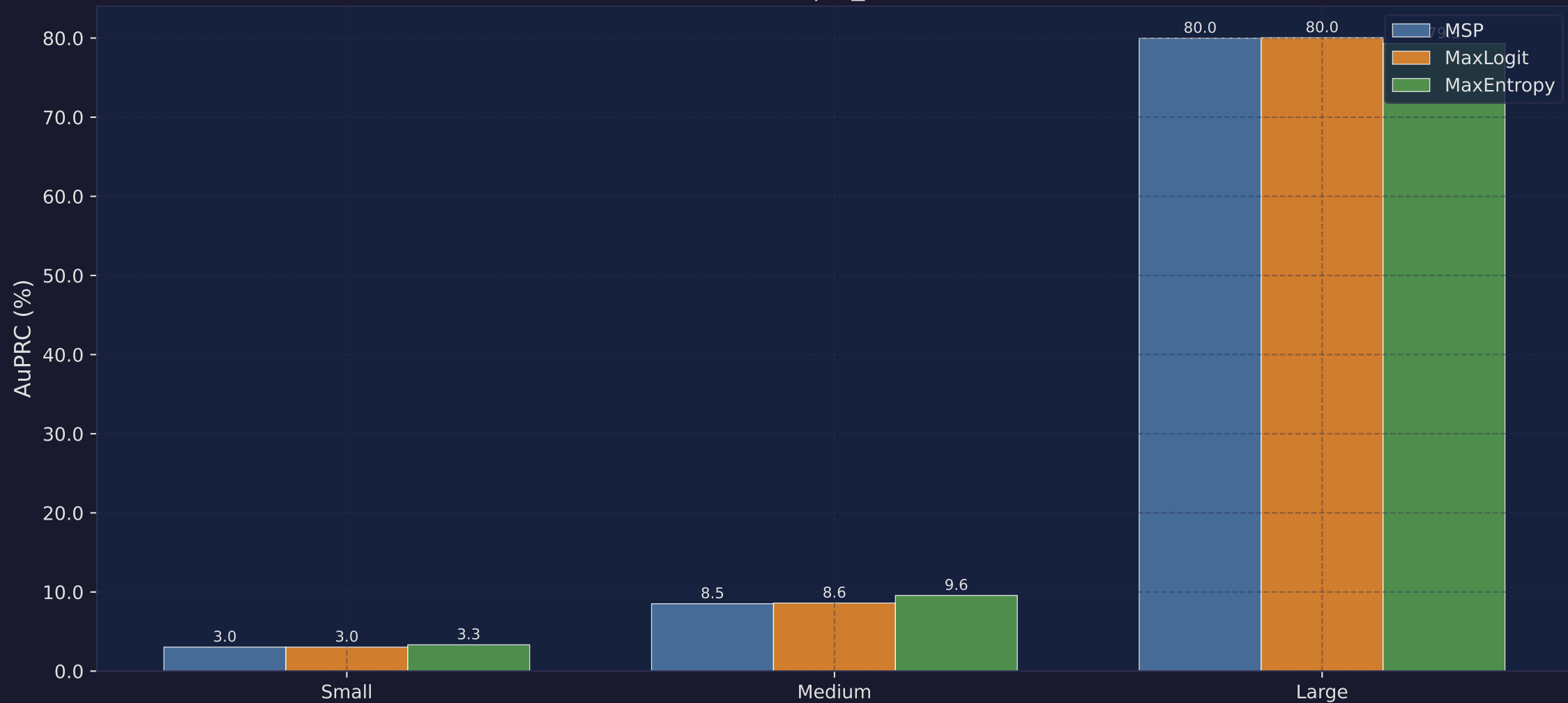
AuPRC by Anomaly Size Bucket EoMT | fs_static
