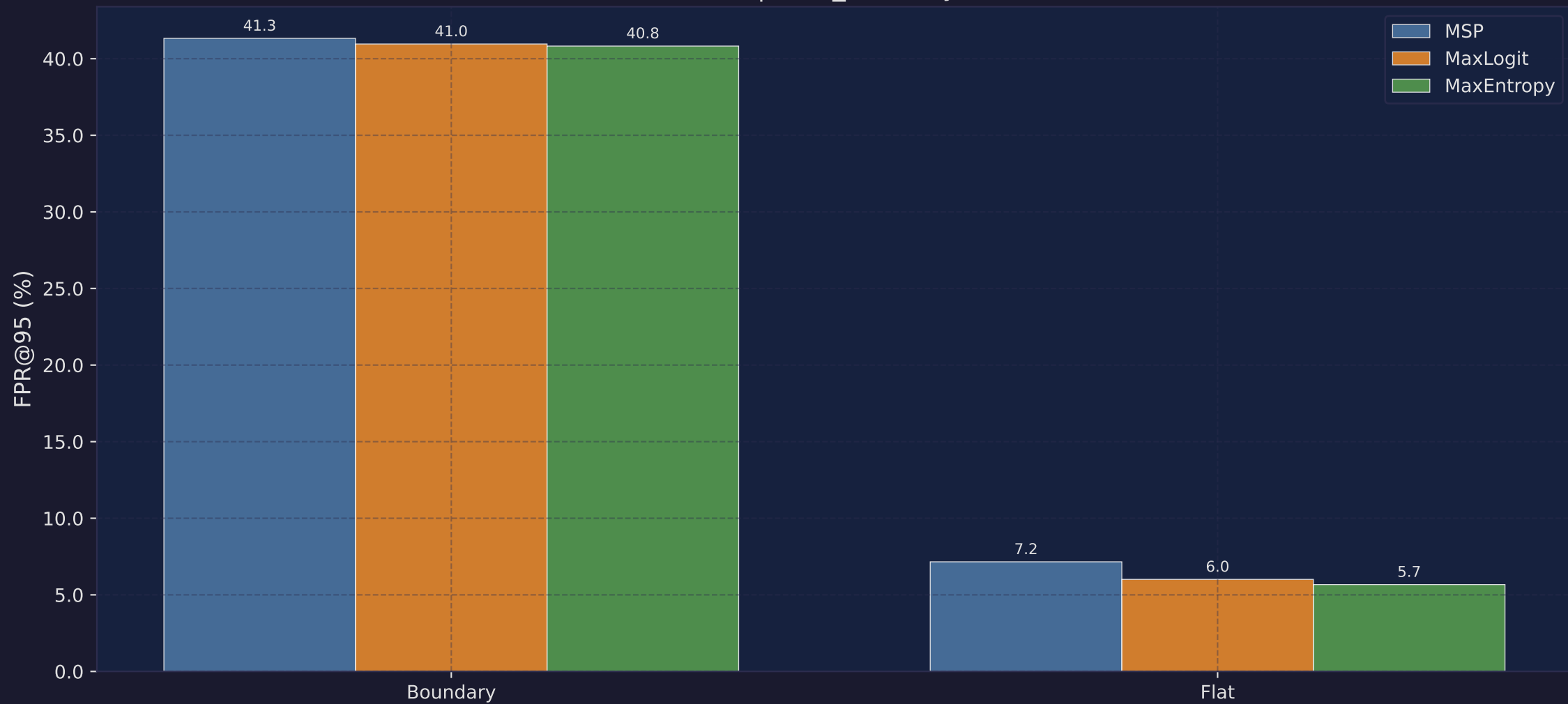
FPR@95 — Boundary vs Flat Region EoMT | road_anomaly21
